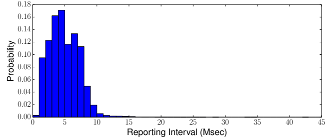
Figure 4: Sensor Event Time Histogram
