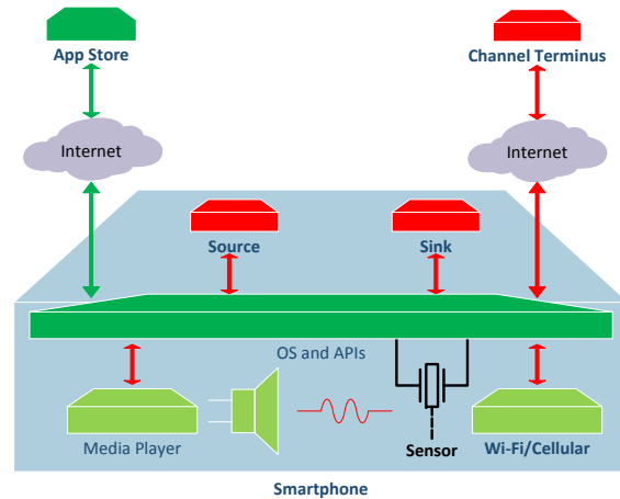
Figure 2: Single Device Covert Communications Channel System Design
