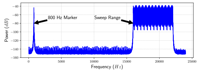
Figure 3: Spectral Components Illustration, Channel Identification Sweep Pattern
